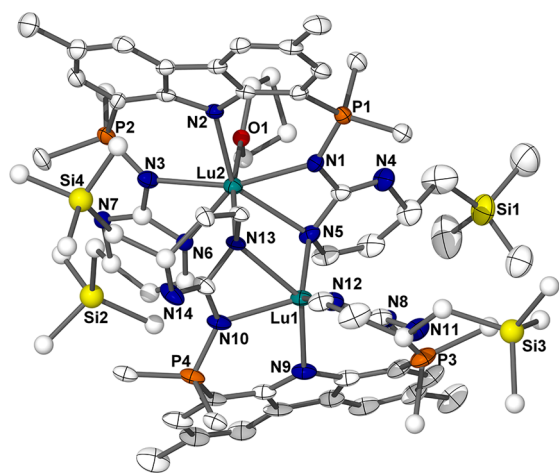
Figure 2. Thermal ellipsoid plot (30% probability) of 3 with hydrogen atoms and P-phenyl rings (except for ipso carbons) omitted for clarity. Positionally disordered atoms are depicted as spheres of arbitrary radius. Selected bond distances (Å) and angles (deg): Lu2–N2 = 2.412(5), Lu2–N3 = 2.297(6), Lu2–N1 = 2.321(5), Lu2–N5 = 2.493(6), Lu2–N13 = 2.354(5), Lu2–N6 = 2.389(16), Lu1–N13 = 2.436(5), Lu1–N10 = 2.264(6), Lu1–N5 = 2.315(6), Lu1–N9 = 2.327(5), Lu1–N8 = 2.305(6), Lu1–N12 = 2.240(6), O1–Lu2 = 2.341(11), N13–Lu2–O1 = 170.2(4), N3–Lu2–N2 = 81.4(2), N2–Lu2–N1 = 81.0(2), N1–Lu2–N5 = 56.4(2), N5–Lu2–N6 = 87.2(5), N6–Lu2–N3 = 53.8(5), N12–Lu1–N5 = 129.0(2), N12–Lu1–N10 = 105.1(2), N12–Lu1–N9 = 118.1(2), N9–Lu1–N10 = 81.1(2), N10–Lu1–N5 = 110.7(2), N9–Lu1–N5 = 102.6(2), N8–Lu1–N13 = 138.6(2).
