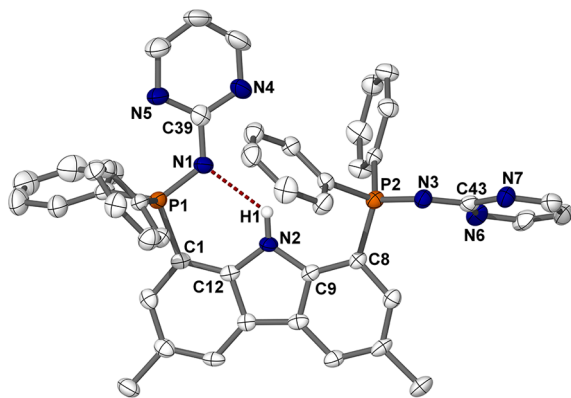
Figure 1. Thermal ellipsoid plot (50% probability) of HL ( 1 ) with hydrogen atoms (except H1) and two chloroform- d solvent molecules omitted for clarity. Selected bond distances (Å), angles (deg), and torsion angles (deg): P1–N1 = 1.597(3), P2–N3 = 1.592(3), N2 \cdots N1 = 2.838(5), N1–P1–C1 = 103.4(2), N3–P2–C8 = 114.7(2), N1–P1–C1–C12 = 33.6(4), N3–P2–C8–C9 = 159.1(3).
