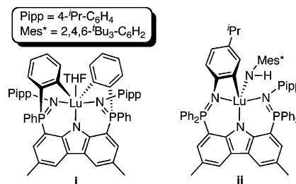
Chart 1. Cyclometalation of a Bis(phosphinimine)carbazole Ligand
