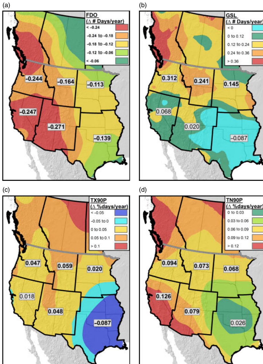
Figure 5. Spatial interpolation of calculated trends in temperature indices across WNA. Regional mean trends calculated using station-specific trends and are overlaid their respective regions. Bold numbers (i.e. -0.244 ) were found to be significant at the p < 0.001 level. This figure is available in colour online at wileyonlinelibrary.com/journal/joc
