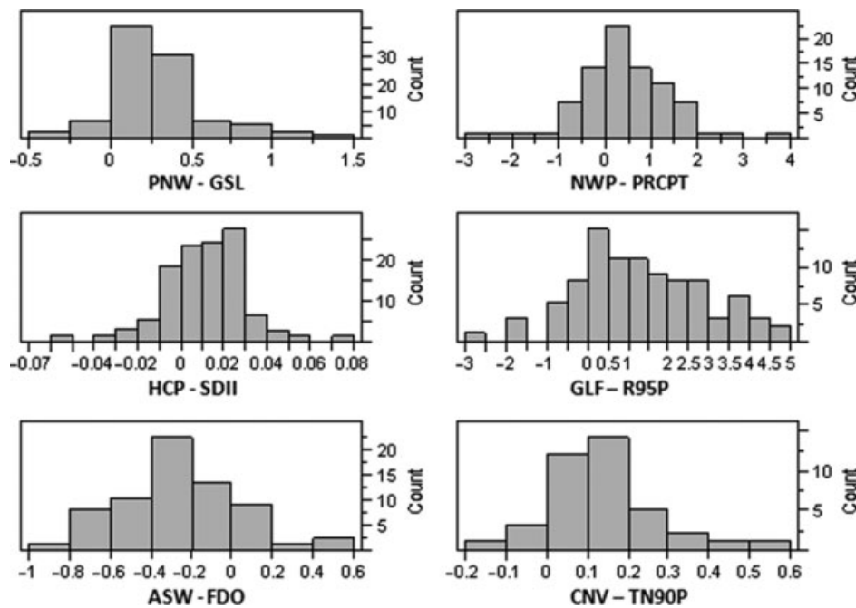
Figure 3. Frequency histograms of weather station trend slopes for the period 1950–2005, for selected climate indicator over each region in western North America.
