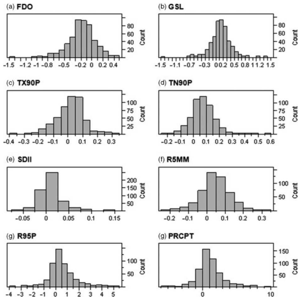
Figure 2. Frequency histograms of weather station trend slopes for the period 1950–2005, for each climate indicator over western North America.
