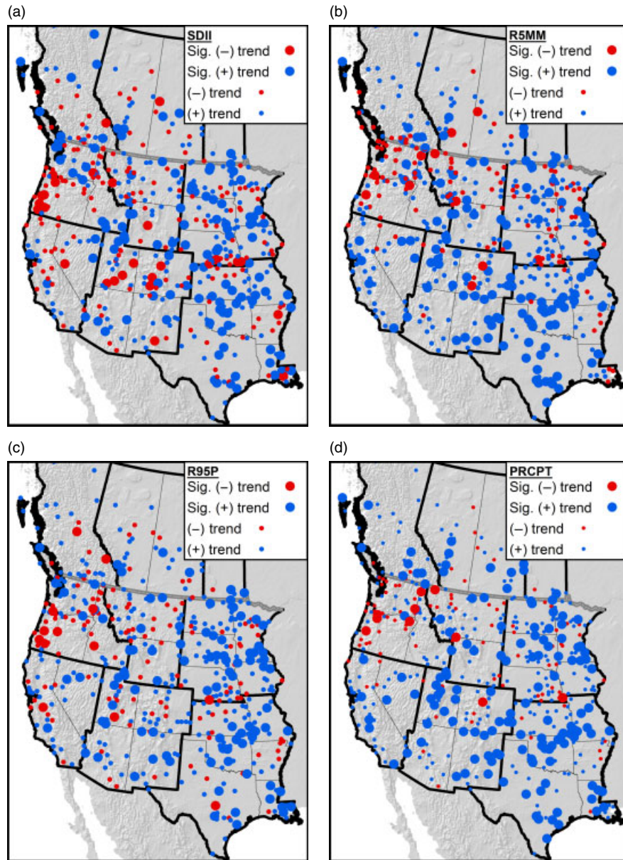
Figure 6. Calculated trends in precipitation indices across WNA by station. Blue points indicate increasing precipitation trends and red dots indicate decreasing precipitation. Larger points are significant at the p < 0.1 level. This figure is available in colour online at wileyonlinelibrary.com/journal/joc
