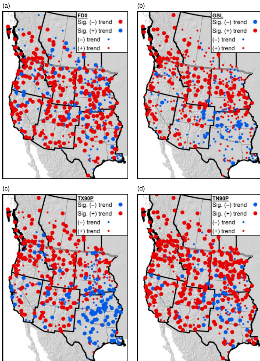
Figure 4. Calculated trends in temperature indices across WNA by station. Red points indicate warming trends and blue dots indicate cooling. Larger points are significant at the p < 0.1 level. This figure is available in colour online at wileyonlinelibrary.com/journal/joc
