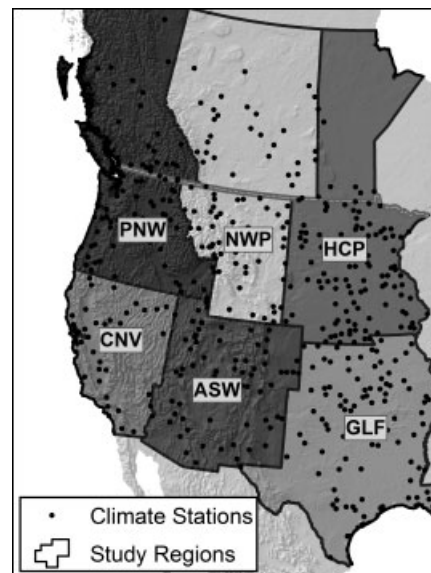
Figure 1. Study area map showing regional classification system and locations of climate stations used. Regions (clockwise from top left): Pacific northwest (PNW), northwest plains (NWP), humid-continental plains (HCP), Gulf (GLF), American southwest (ASW), California–Nevada (CNV).
