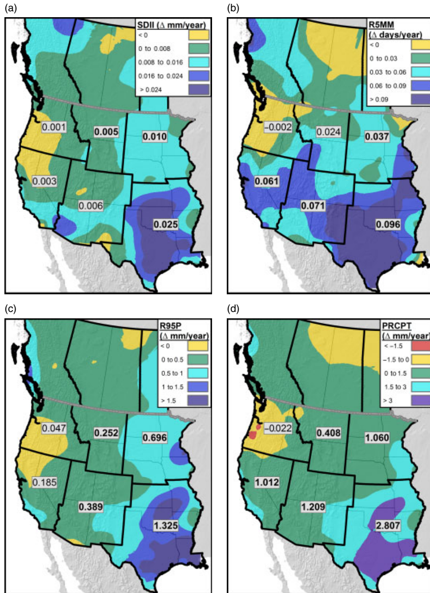
Figure 7. Spatial interpolation of calculated trends in precipitation indices across WNA. Regional mean trends calculated using station-specific trends and are overlaid their respective regions. Bold numbers (i.e. 0.025 ) were found to be significant at the p < 0.001 level. This figure is available in colour online at wileyonlinelibrary.com/journal/joc
