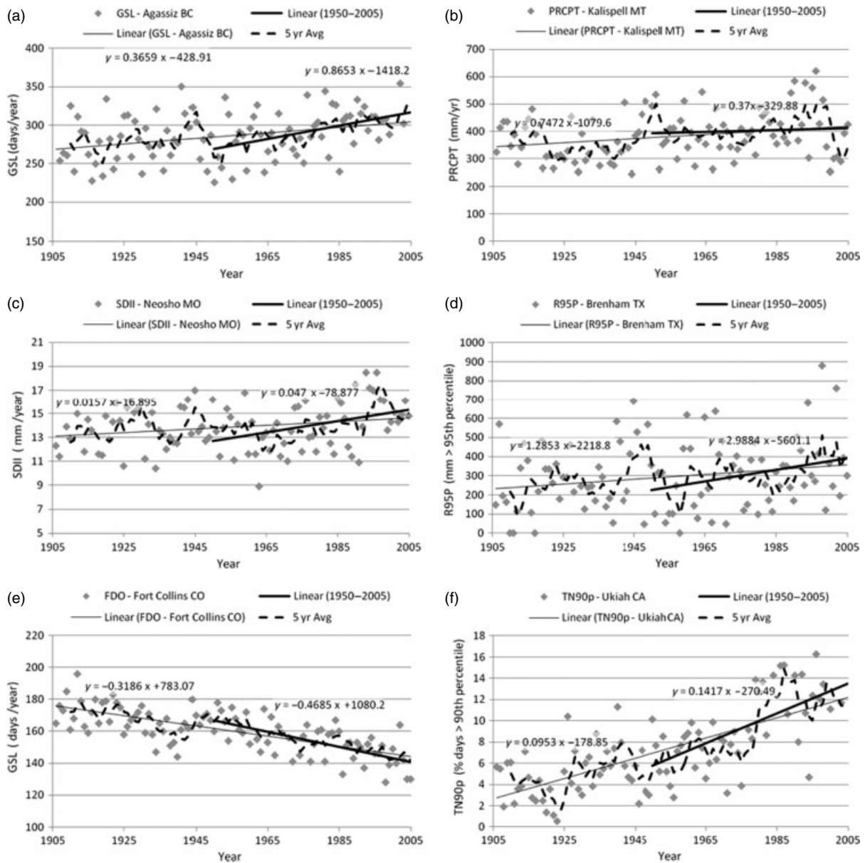
Figure 9. The 100-year station-specific time series. Trend analysis was performed for all indices for selected climate stations with high quality long-term records; 1906–2005 linear trends are shown with thin solid line; 1950–2005 linear trends are shown with bold solid line; 5-year moving averages are shown with dashed line.
