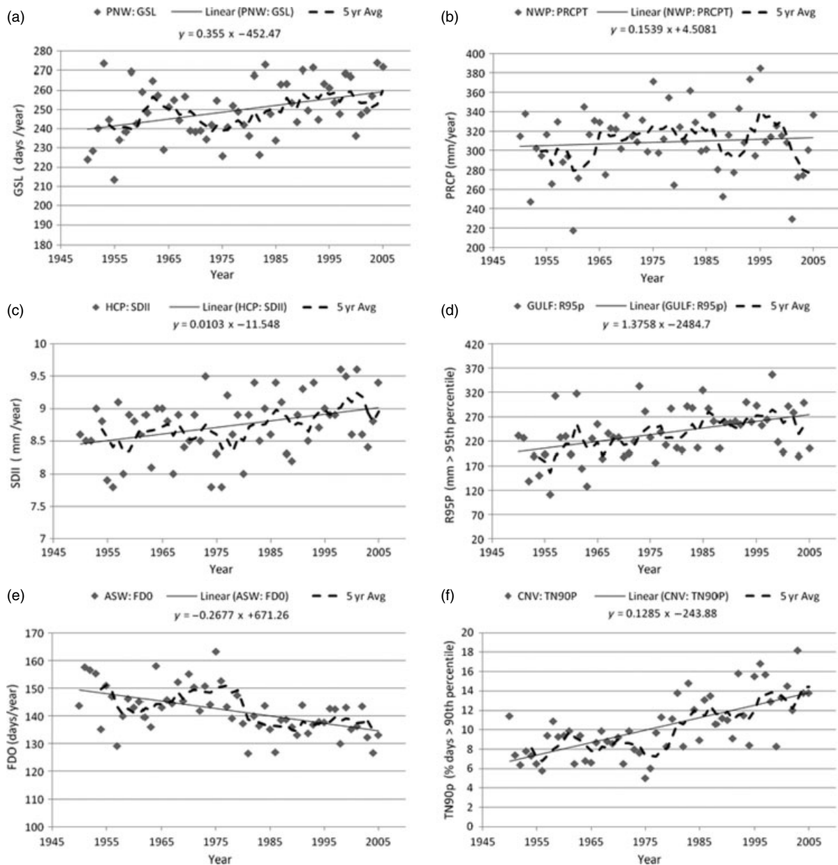
Figure 8. Regional mean time series for selected indices. Annual mean index counts were calculated for each index in each region and plotted over time. Linear trends are shown with solid line. The 5-year moving averages were calculated and are shown with dashed line.
