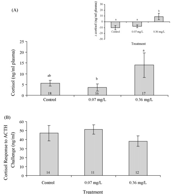
Fig. 2. Plasma cortisol levels and \Delta cortisol (in the inset graph) expressed as change in plasma cortisol levels between day 30 and day 8 (A) and the ability of the head kidney to secrete cortisol (B) in juvenile rainbow trout (mean \pm S.E.) exposed for 30 days to waterborne sodium selenite ( \text{Na}_2\text{SeO}_3 ). Groups with different letters are significantly different (Kruskal–Wallis) in A. No significant differences were observed in B (ANOVA). Sample size indicated in the bars.
